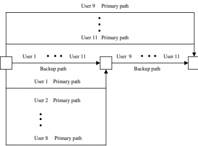
Fig. 5. Network Topology.
