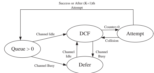
Figure 1: The State Diagram for an IEEE 802.11 Node.
