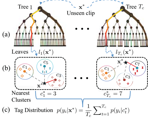
Figure 3. Structure-driven non-visual tag inference: (a) Channel an unseen clip x^* into individual trees; (b) Estimate the nearest clusters of x^* within the leaves it falls into: hollow circles denote clusters; (c) Compute the tag distributions by averaging tree-level predictions.
