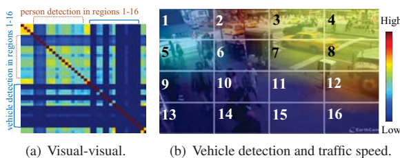
Figure 10. The latent correlations among heterogeneous visual and multiple non-visual sources discovered on the TISI dataset.
