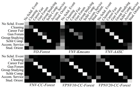
Figure 7. Tag inference confusion matrices on the ERCe dataset.
